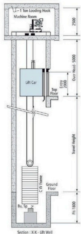
Hoistway Elevation Drawing
